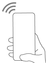
FusionSolar App
