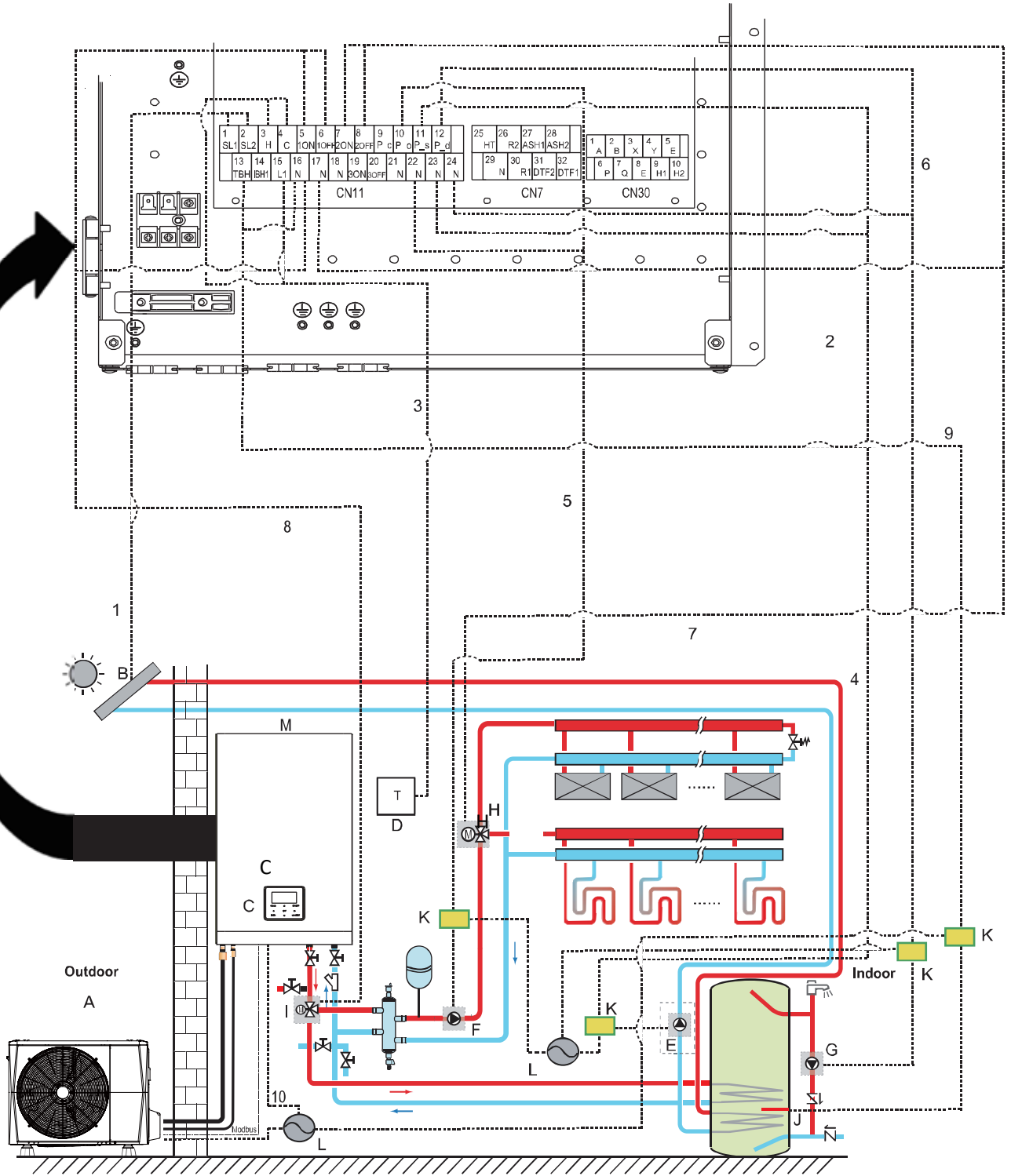
Figure 3-5.1: Wiring overview
