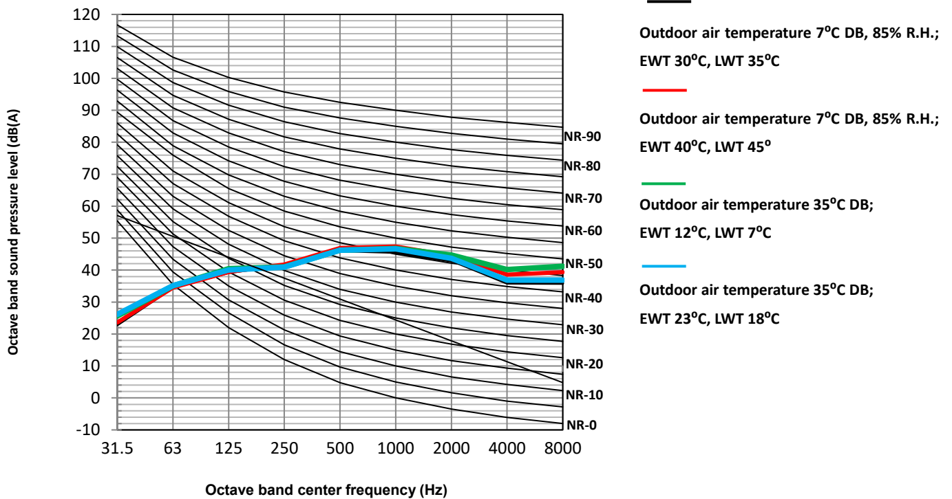
Figure 2-7.4: KHA-12RY3-B octave band levels
