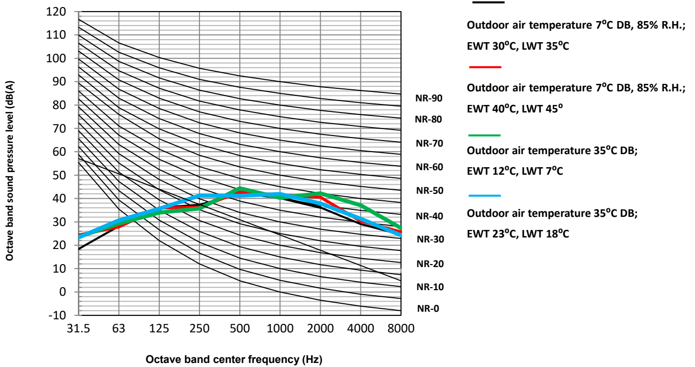
Figure 2-7.1: KHA-06RY1-B octave band levels
