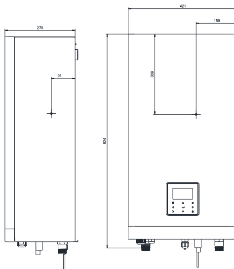
Figure 2-3.3: Dimensions and center of gravity (unit: mm)
