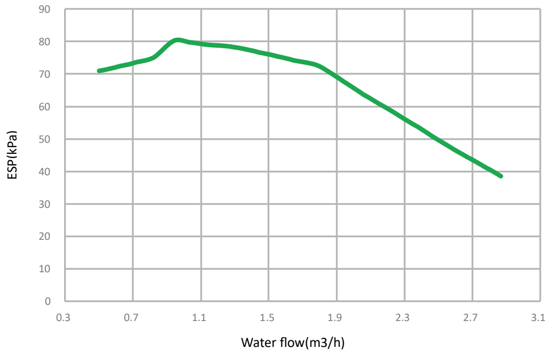
Figure 2-6.2: KMK-160RY3 hydronic performance
