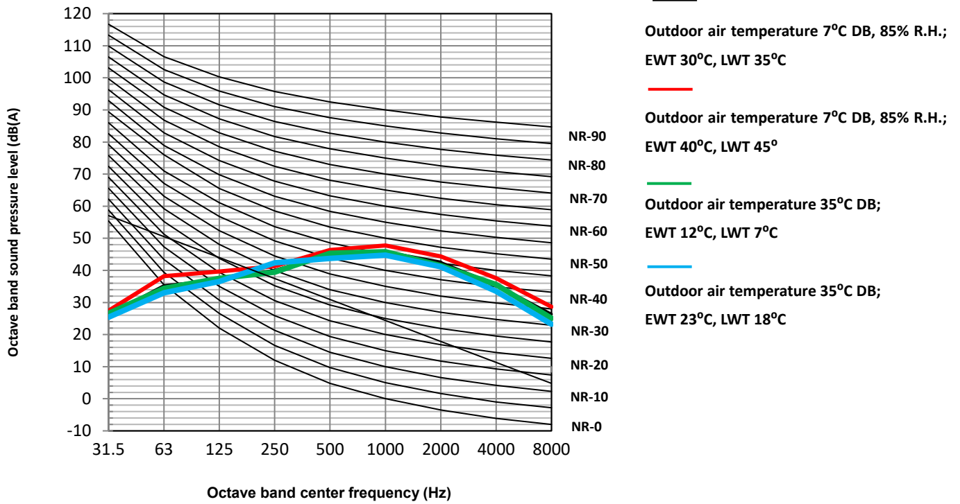
Figure 2-7.3: KHA-10RY1-B octave band levels
