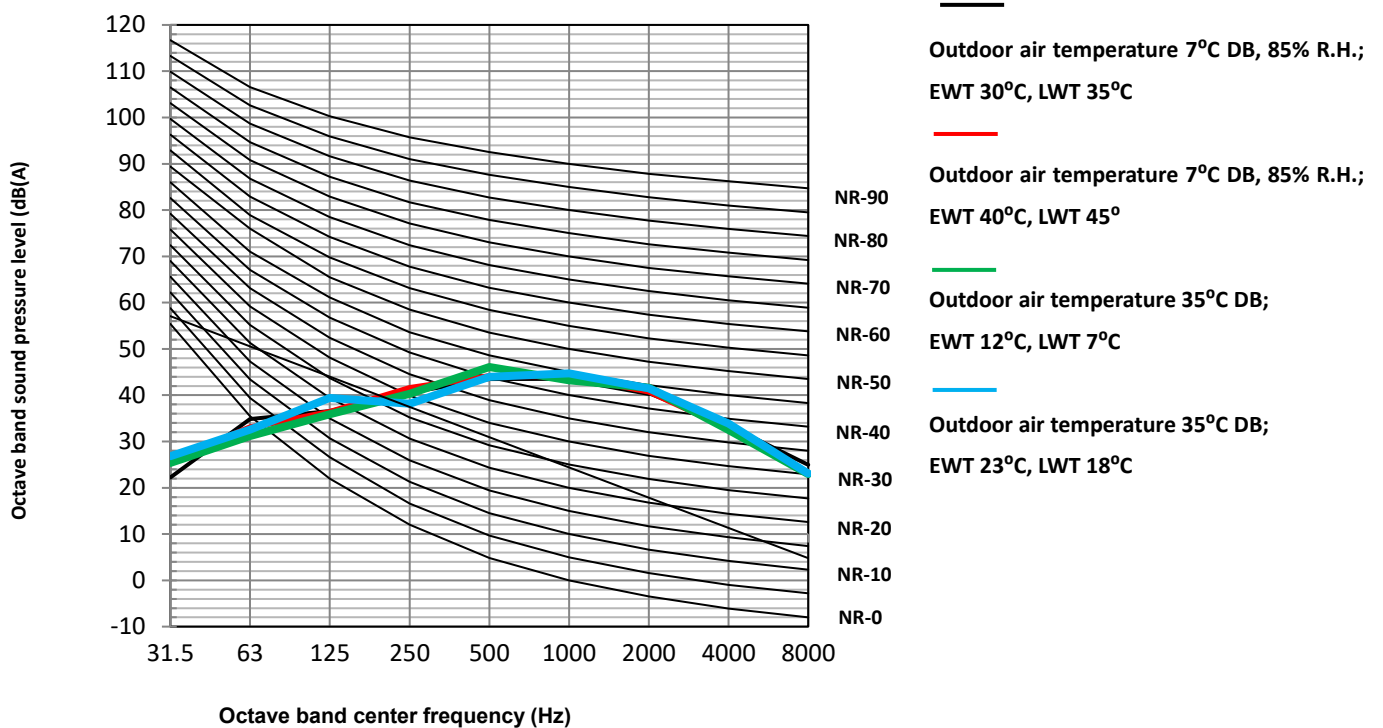
Figure 2-7.2: KHA-08RY1-B octave band levels
