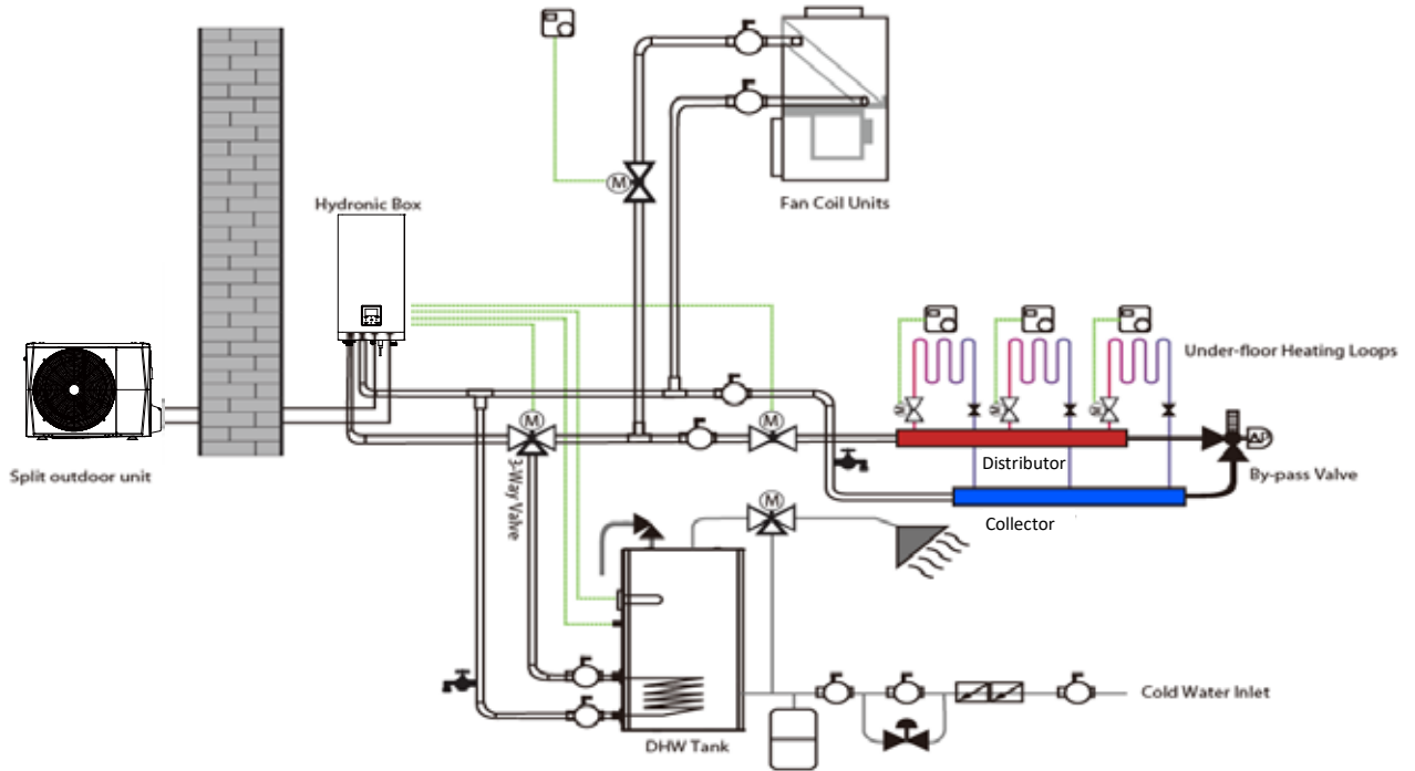
Figure 1-1.1: System schematic
