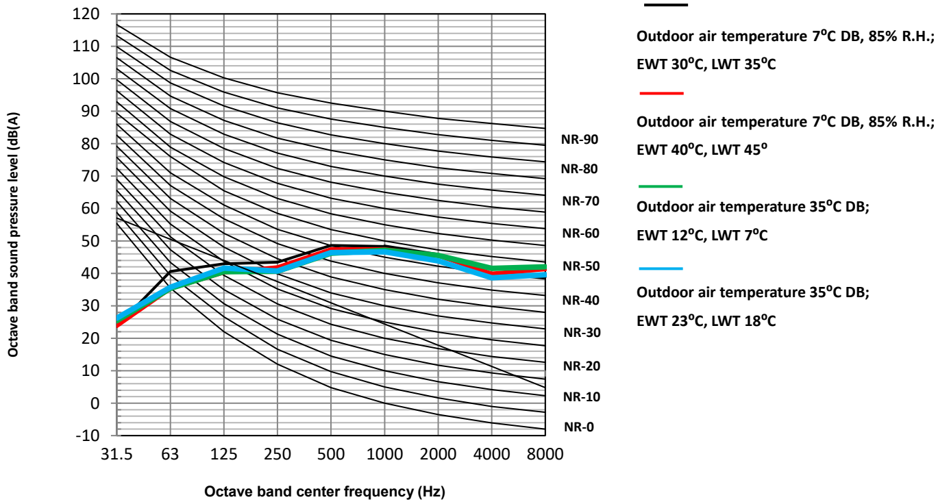
Figure 2-7.5: KHA-14RY3-B octave band levels
