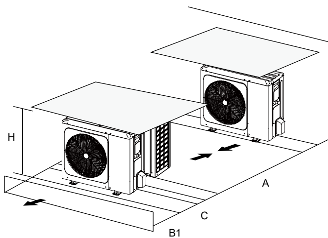
Figure 3-2.10: Single row installation
