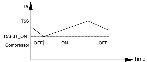
Figure 3-8.5: dT5_ON
