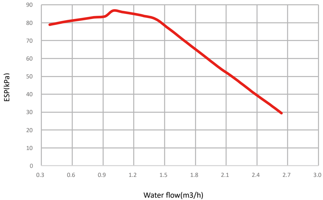
Figure 2-6.1: KMK-60RY1, KMK-100RY3 hydronic performance
