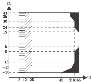
Figure 2-5.3: Domestic hot water operating limits 1
